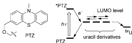
Figure 2. Chemical structure of phenothiazine (PTZ). Excess electrons injected from photoexcited PTZ (PTZ*) migrate through T and U derivatives and react irreversibly with Br U or recombine with the PTZ radical cation (PTZ + ).
