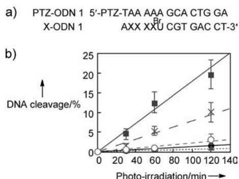
Figure 3. EET from photoexcited PTZ to Br U through four uracil derivatives (X). a) DNA sequences of PTZ-ODN1 and X-ODN1; b) 32 P-radiolabeled duplex DNA (PTZ-ODN1/X-ODN1; X = (●) T, (×) U, (■) F U, (▲) OH U, (○) P U) in buffer solution (10 mM phosphate, 90 mM NaCl, pH 7.0) was exposed to UV light (365 nm) for the indicated periods at 4 °C, followed by treatment with piperidine at 90 °C for 30 min. DNA fragments that corresponded to electron-transfer products were quantified using PAGE.
