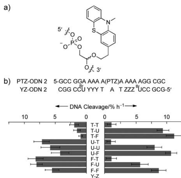
Figure 4. Asymmetrical EET from photoexcited PTZ to Br U through uracil derivatives. a) Chemical structure of ( R )- and ( S )-PTZ inserted in the middle of oligodeoxynucleotides; b) 32 P-radiolabeled duplex DNA (( R )-PTZ-ODN2/YZ-ODN2; Y, Z = T, U, F U) in buffer solution (10 mM phosphate, 90 mM NaCl, pH 7.0) was exposed to UV light (365 nm) at 4 °C, followed by piperidine treatment.
